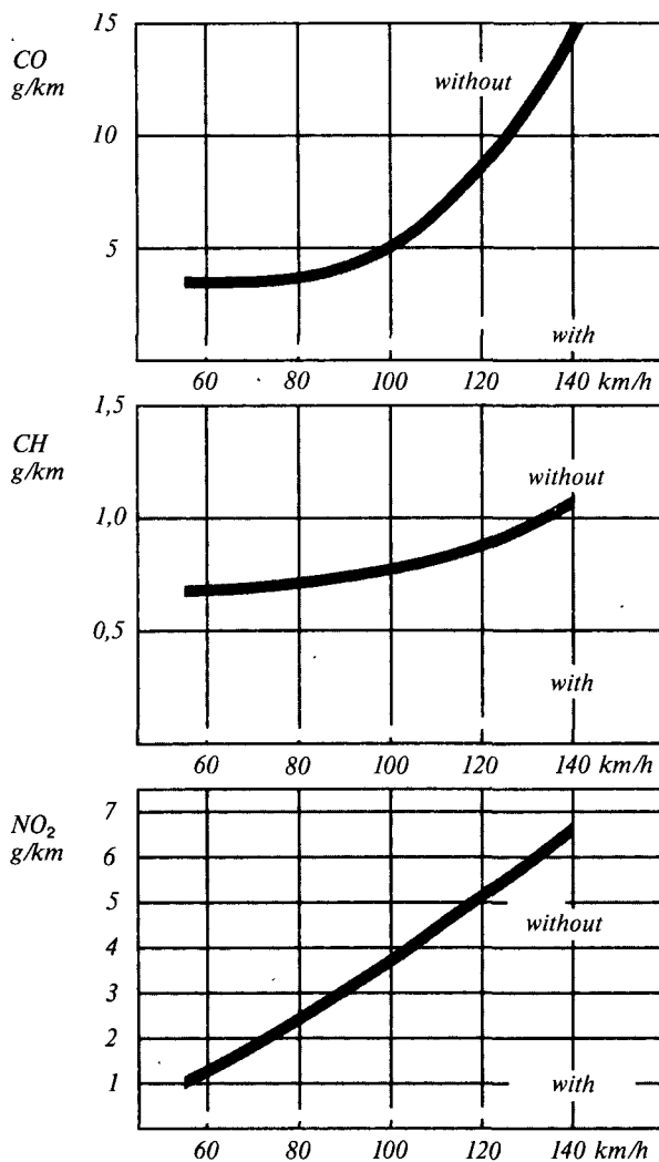
Pollution emitted by a medium-sized car with and without a catalytic converter
